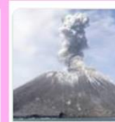
Krakatoa 813 m
